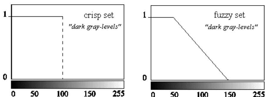
Fig. Representation of “dark gray-levels” with a crisp and a fuzzy set
