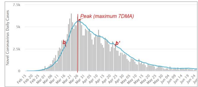
Figure 3: The daily new cases in 7DMA for Italy. Here b and b' represent 50% of the peak before and after the peak resp. Notice that number of days from pint b to the peak is denoted as d_2 .
